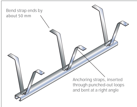
Anchor channel JSA with installed straps.
