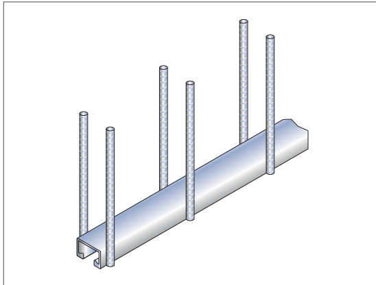
Anchor channel type JRA with reinforcing steel anchors welded on both sides.
