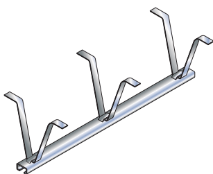
JORDAHL® Anchor Channels JSA
