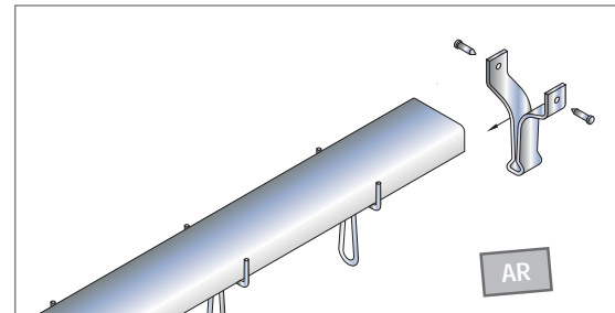
JTB-AR channel with JTB-EA end anchors.
