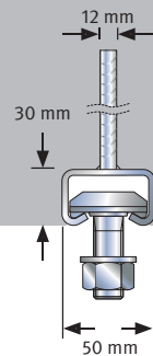
JGB K 50/30 N_{Rd} = V_{Rd} = 17.2 \text{ kN}
