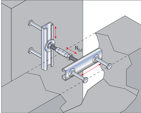
Turnbuckle Connections JSV provide three-dimensional alignment.
