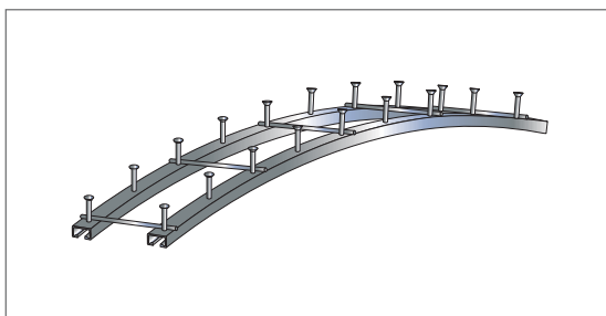
Curved anchor channel pair with welded-on spacers.
