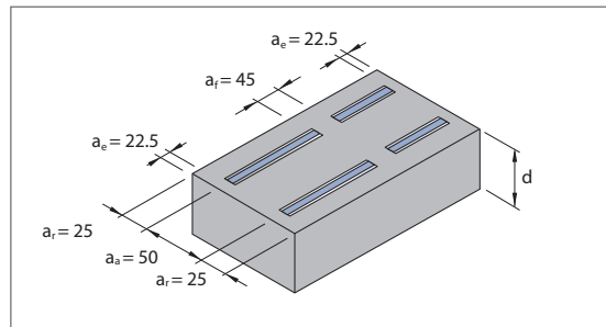
Associated edge distances [cm].
