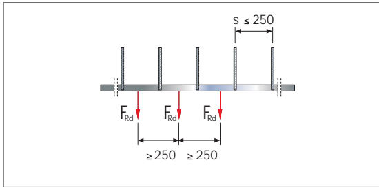
Load arrangement, single load.
