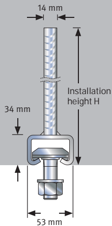
JGB K 53/34 N_{Rd} = V_{Rd} = 30.6 \text{ kN}
