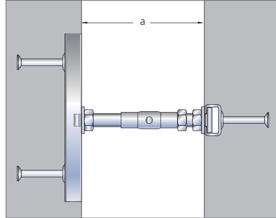
Installation overview.
