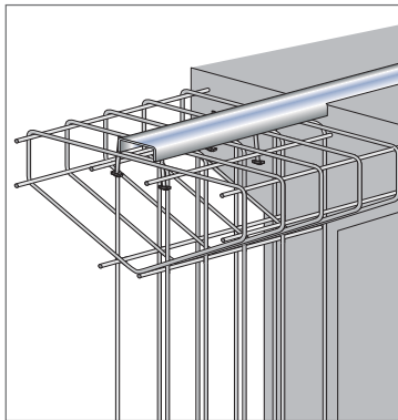
Installation in heavily reinforced elements
