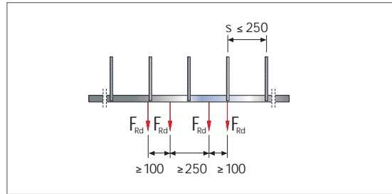
Load arrangement, load pairs.
