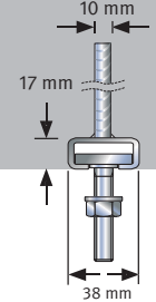
JGB K 38/17 N_{Rd} = V_{Rd} = 10.0 \text{ kN}
