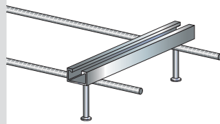
JORDAHL® Facade Connection Channels JTA-RT
