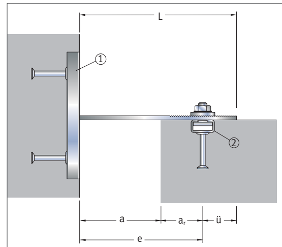
Installation overview.
