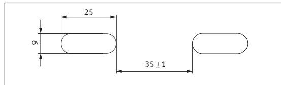
Standard slot pattern 9 x 25
