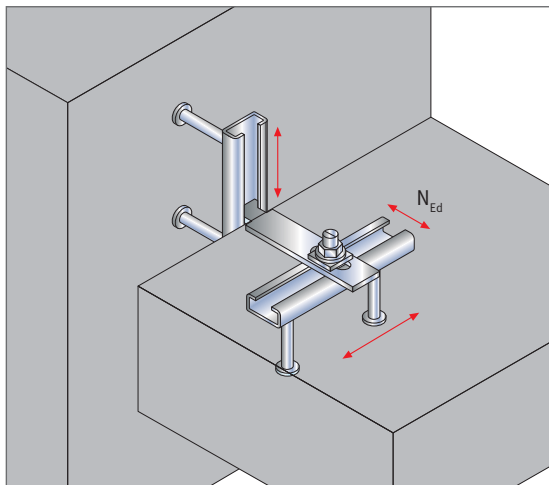
JORDAHL® toothed straps JVB-Z for three-dimensional alignment.
