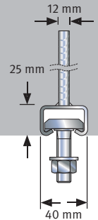
JGB K 40/25 N_{Rd} = V_{Rd} = 11.1 \text{ kN}
