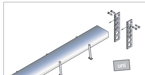
JTB-uni channel with JTB-EB end anchors.
