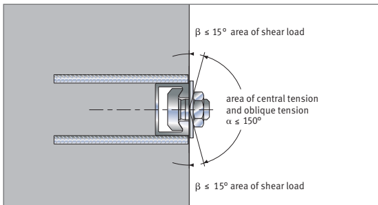
Load ranges.
